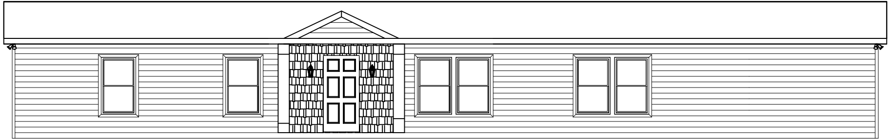
FRONT ELEVATION 10' DORMER OPTION
